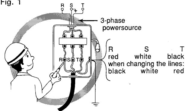
Power Cable
